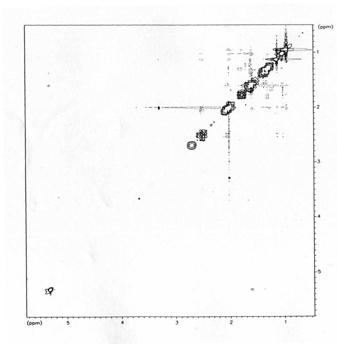
Phase- sensitive NOESY spectrum of paesslerin A.
