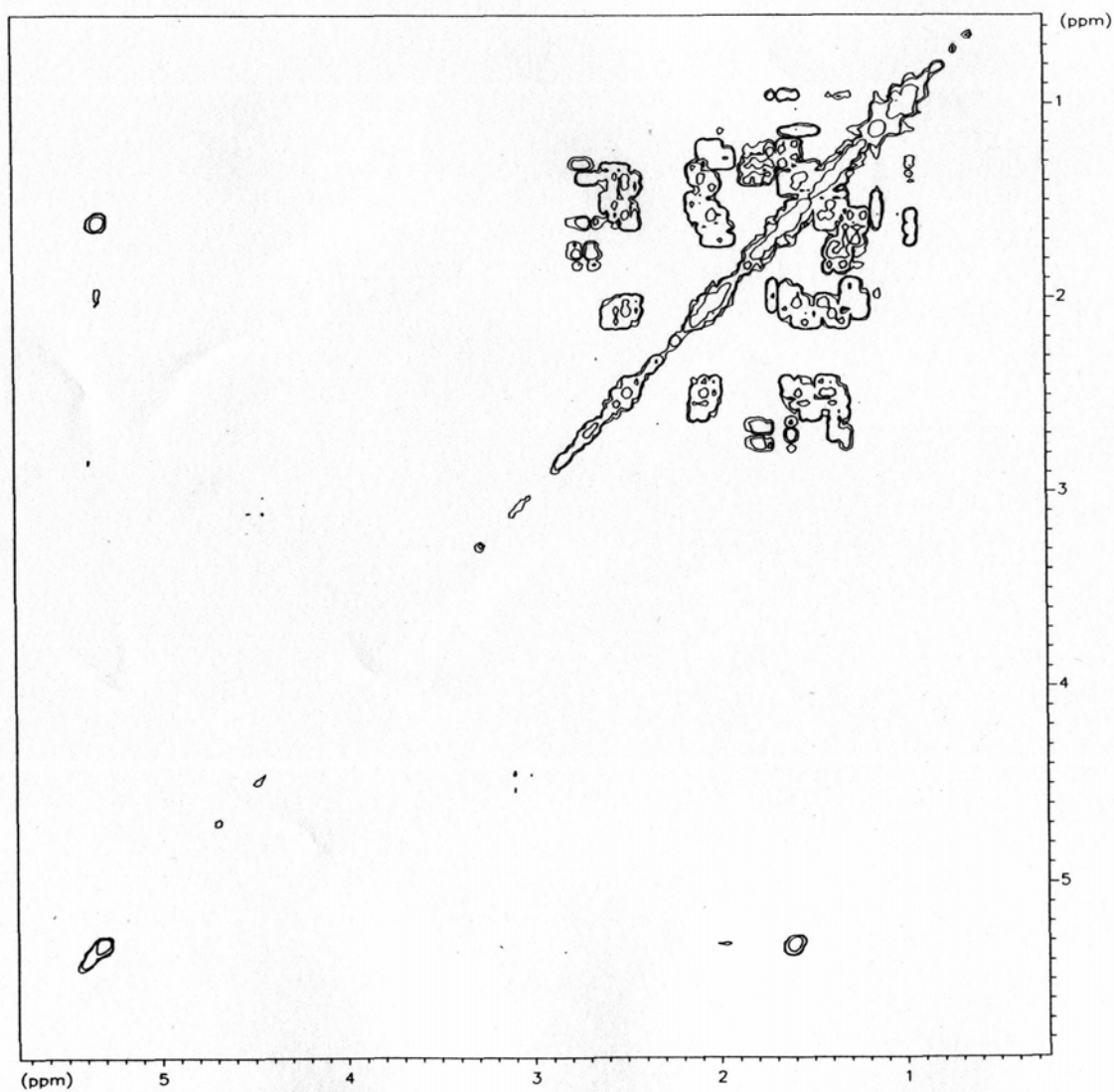
COSY ^1\text{H} - ^1\text{H} spectrum of paesslerin A.
